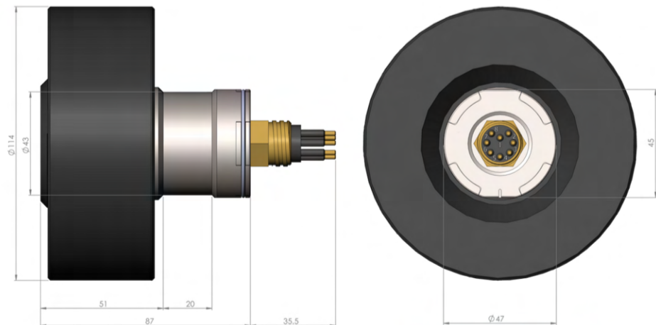
Dimensions given in mm.
